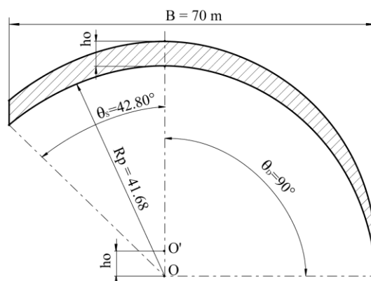
Fig. 1 – Geometric dimensions that characterize the volume of the cut.
