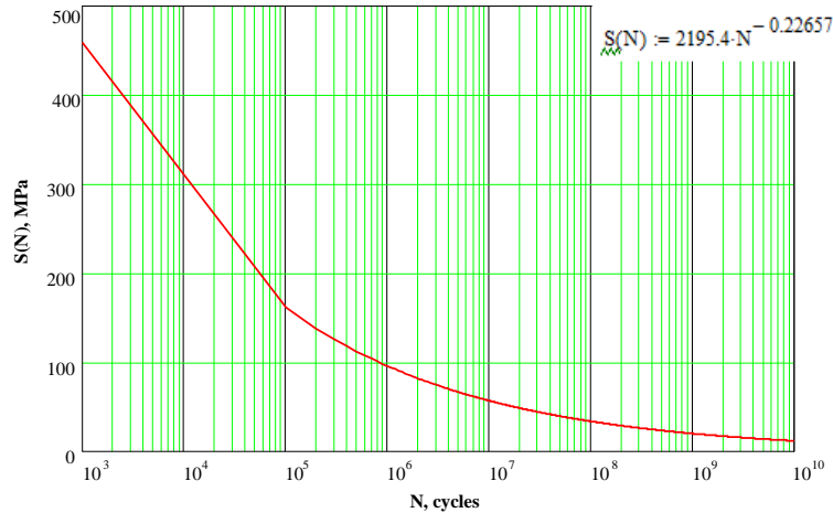
Fig. 7 – The fatigue curve of the material which constitutes the truss.
