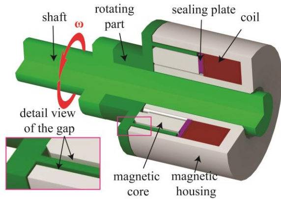
Fig. 2 – Axonometric view of MRB. The rotating part includes the cylindrical geometry and the shaft colored with green on figure.
