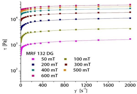
Fig. 3 – Flow curves determined for MRF132DG for several magnetic flux density values from 50 mT to 600 mT.
