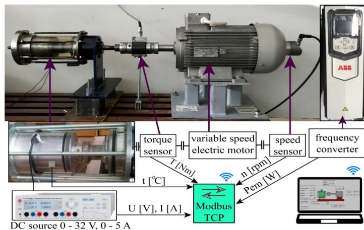
Fig. 6 – Test rig developed to assess MRB's performances available at University Politehnica Timisoara.
