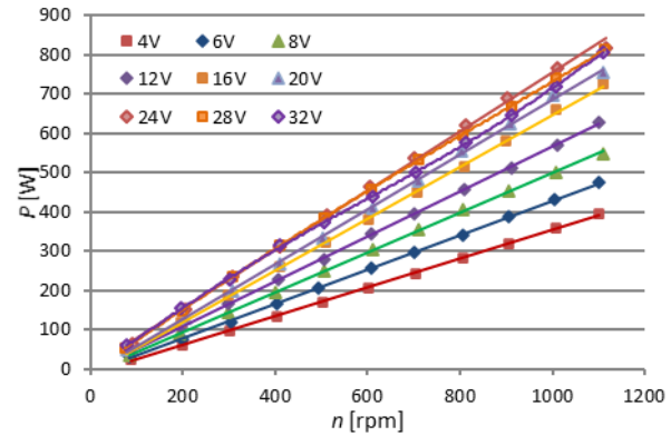
Fig. 8 – Braking power ( P [W]) provided by MRB for voltage values up to 32V over range speed from 100 rpm to 1100 rpm.
