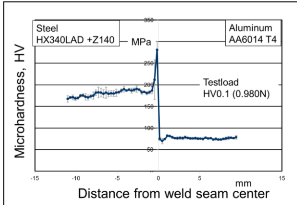
Fig. 2 Microhardness Measurement
