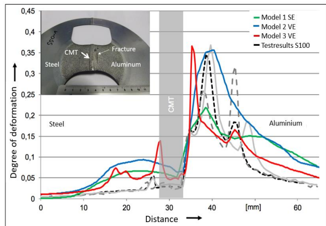
Fig. 11 Modelling types
