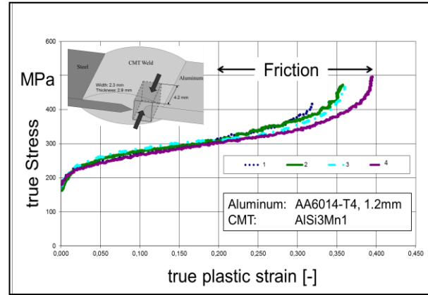
Fig. 3 Stress-Strain curves
