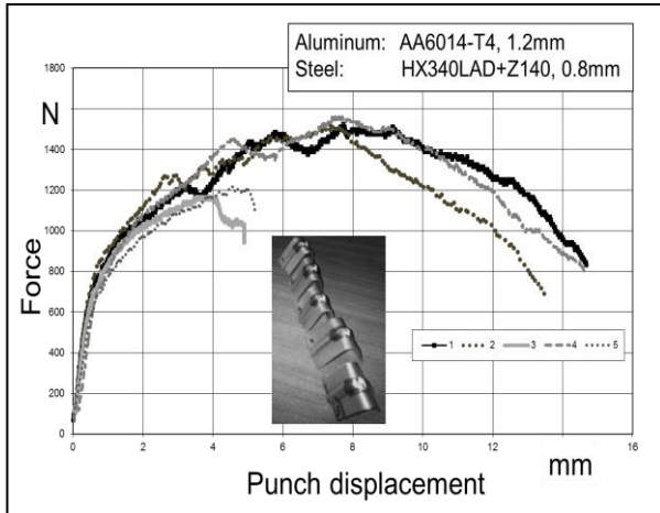
Fig. 5 Three Point bending test
